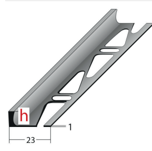
End-edge, straight, silver anodized Art.-Nr. Z 511/anodized
