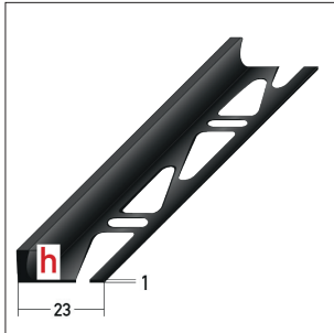
End-edge, straight, black anodized Art.-Nr. Z 511/black
