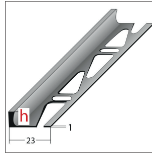
End-edge, straight * Art.-Nr. Z 511
