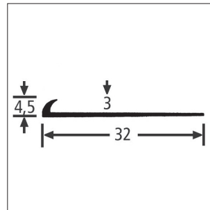
PVC-end profile Art.-Nr. Z 180
