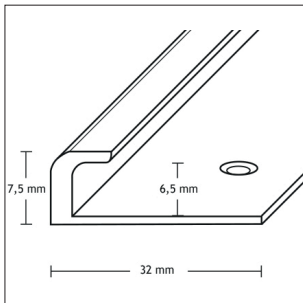
PVC-end profile Art.-Nr. Z 172
